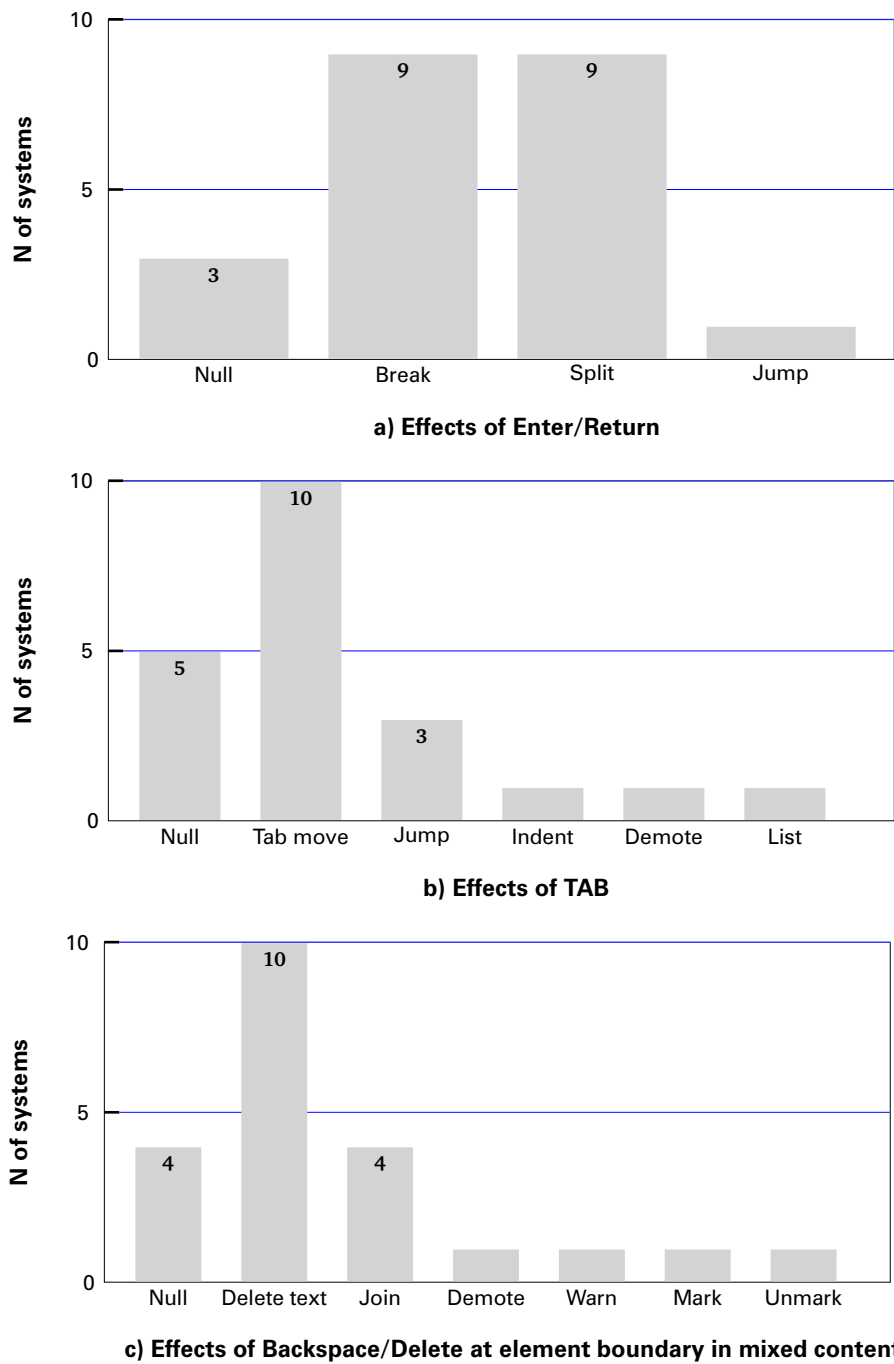
Figure 3.14: Software analysis: summary of editing character behaviour
